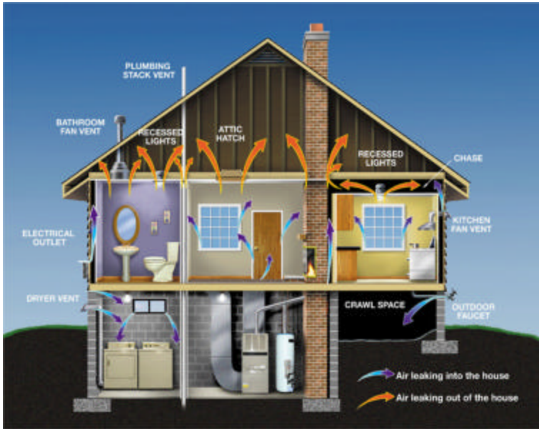
HOT & COLD AIR LEAKING IN & OUT OF HOMES
